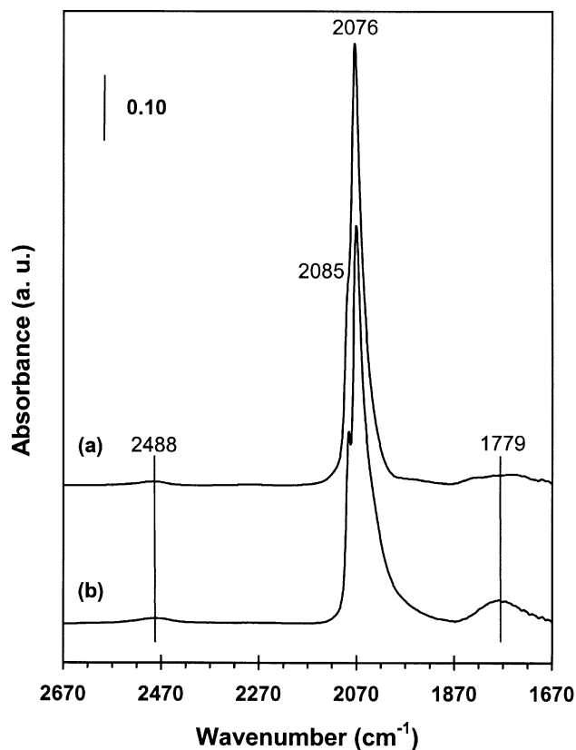
Fig. 6. In situ DRIFTS spectra of CO adsorbed at 300 K on 0.78% Pt/SiO 2 after different pretreatments and a purge with Ar: (a) after pretreatment I; (b) after pretreatment II following H 2 titration at 300 K by flowing 45% H 2 (340 Torr) in Ar.
